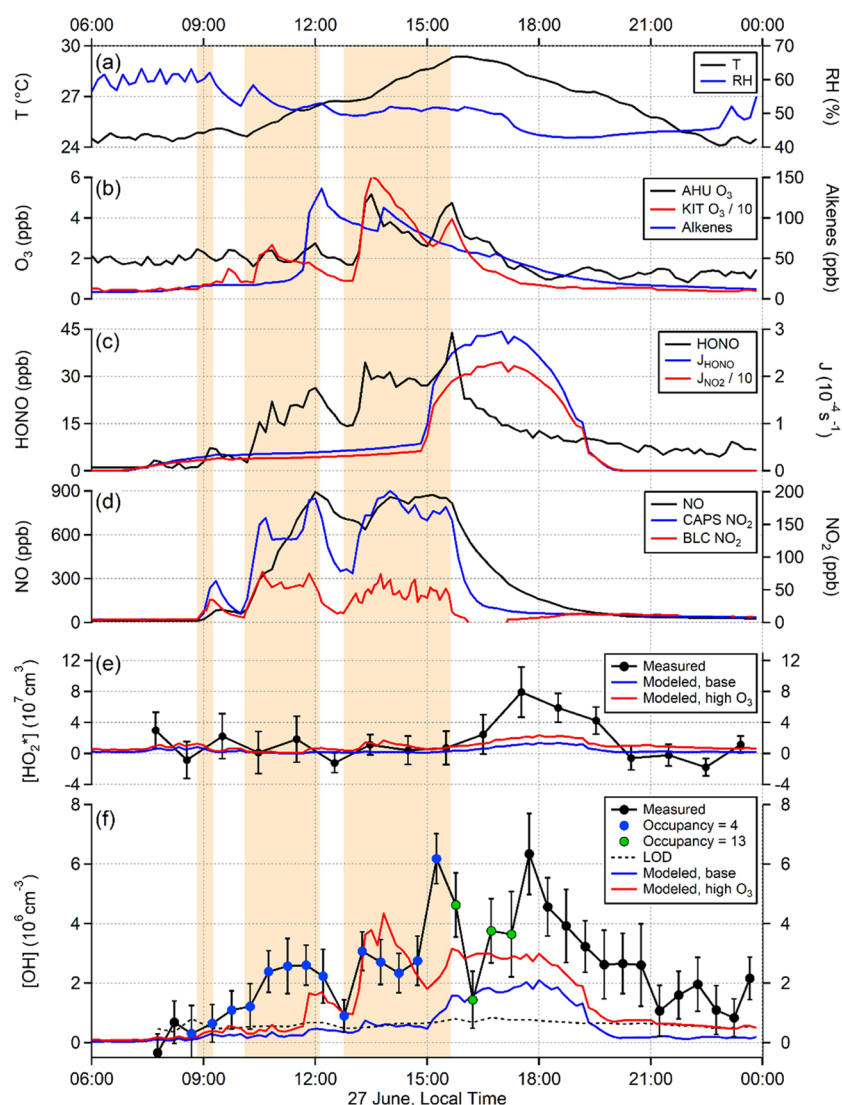
Figure 1. Measurements from the 27 June Thanksgiving experiment. Orange-shaded regions indicate periods of gas cooking. (a) Temperature and relative humidity (b) alkene concentrations and both \text{O}_3 instruments, with the KIT \text{O}_3 divided by 10, (c) HONO and J_{\text{HONO}} , (d) NO and both measurements of \text{NO}_2 , (e) measured \text{HO}_2^* and modeled \text{HO}_2 concentrations from the base and high \text{O}_3 scenarios (see text), and (f) measured and modeled OH concentrations from the base and high \text{O}_3 scenarios. Green points in (f) indicate a period of increased human activity near the OH instrument, potentially creating a local OH sink or sink of photolytic precursors resulting in lower concentrations.
